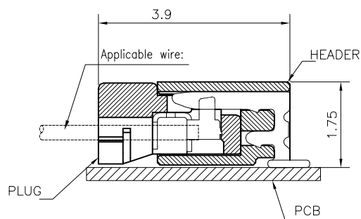
MATED CONDITION
